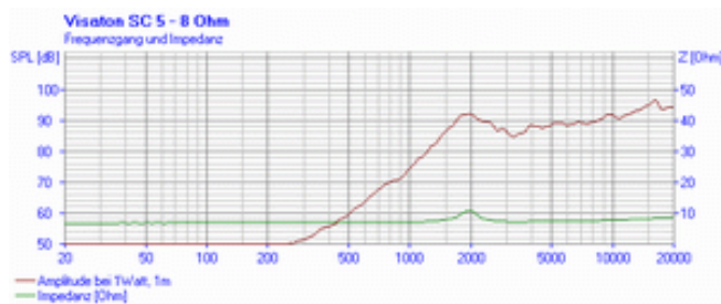
frequency- and impedance response
